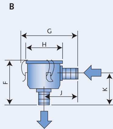
Filter Assembly
