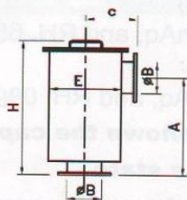
真空過濾筒 FILTER TANK
