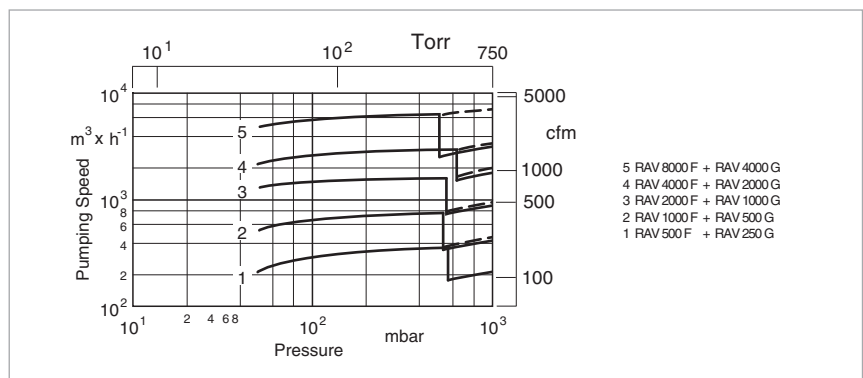
Pumping speed diagram of RAV F + G at 50 Hz
