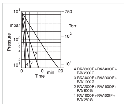
Pump-down time diagram for a 50 m 3 tank for RAV F, F + G at 50 Hz
