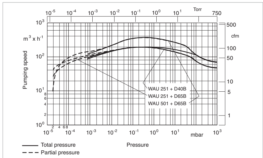
Pumping speed diagram at 50 Hz
