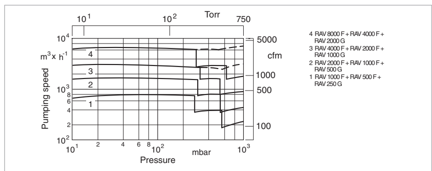
Pumping speed diagram of RAV F, F + G at 50 Hz
